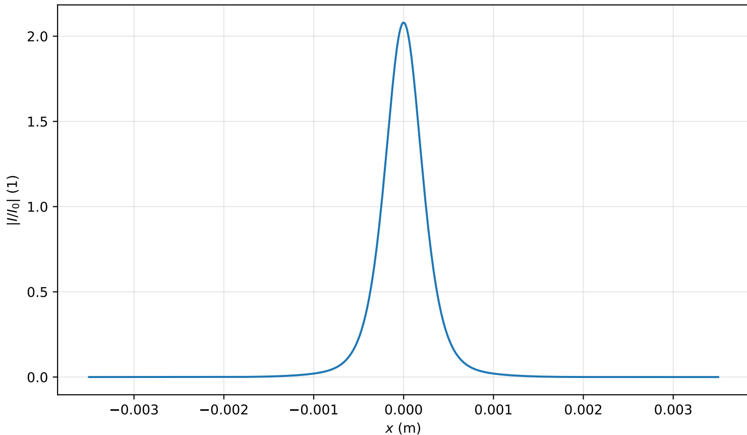
Intensity profile I(x, y = 0, z = 1.911m)/I_0 , P_{in}=1.0P_{cr} , artificial time
